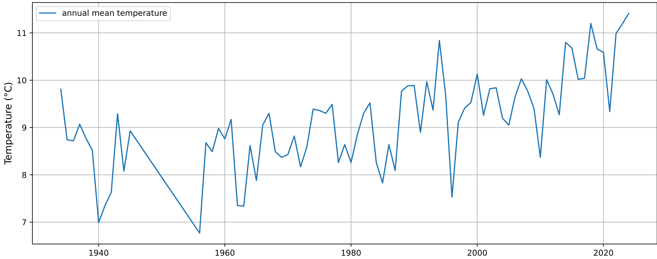
Annual Mean Temperature
